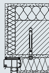
Karpleng Paigaldus ava taha (ainult MZ Thermo)
