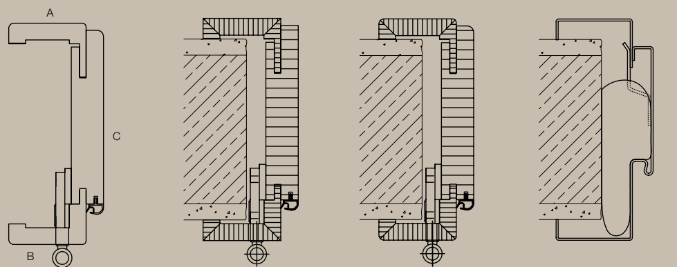
A: Decorative edge Timber frame, angular Timber frame, round edge Steel profile frame VarioFix B: Rebate cladding C: Jamb lining
